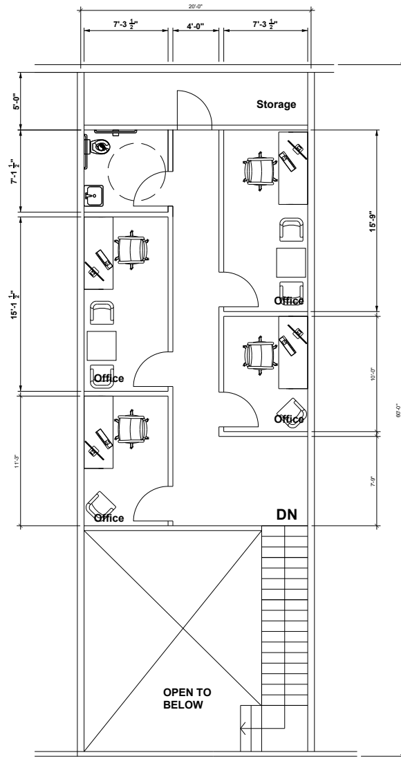
763 S.F. (not counting stairs) SECOND FLOOR
